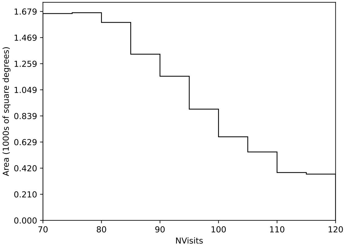
roll_uniform_early_half_mjdp0_v3.4_10yrs Yr 3-4 all bands: NVisits
