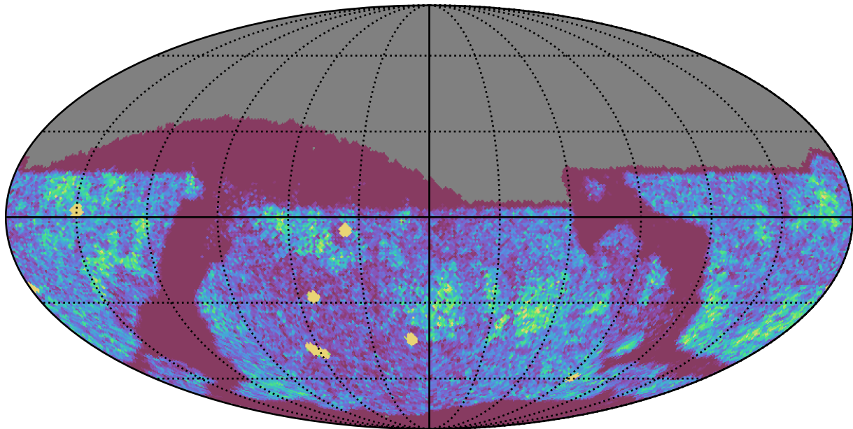
roll_uniform_early_half_mjdp0_v3.4_10yrs Yr 1 z band: NVisits
