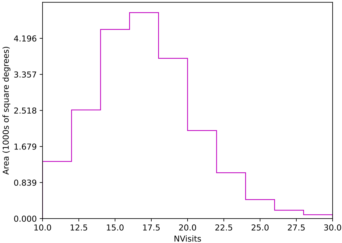
roll_uniform_early_half_mjdp0_v3.4_10yrs Yr 1 z band: NVisits
