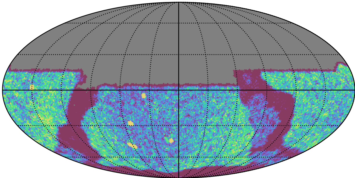
roll_uniform_early_half_mjdp0_v3.4_10yrs Yr 1 y band: NVisits
