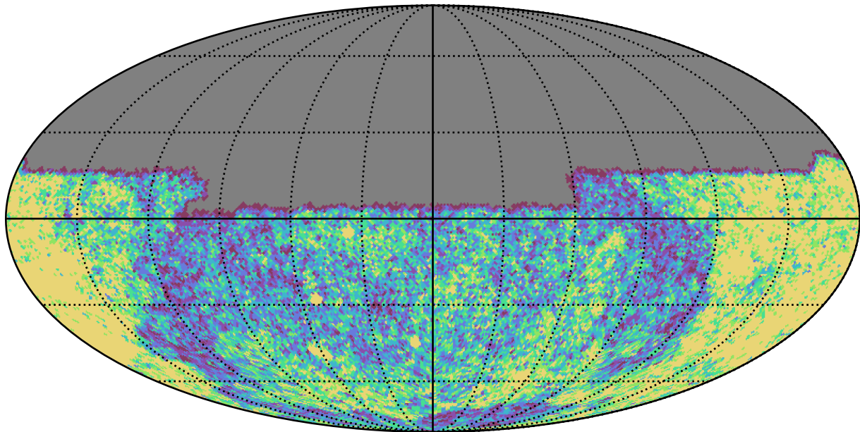
roll_uniform_early_half_mjdp0_v3.4_10yrs Yr 1 u band: NVisits
