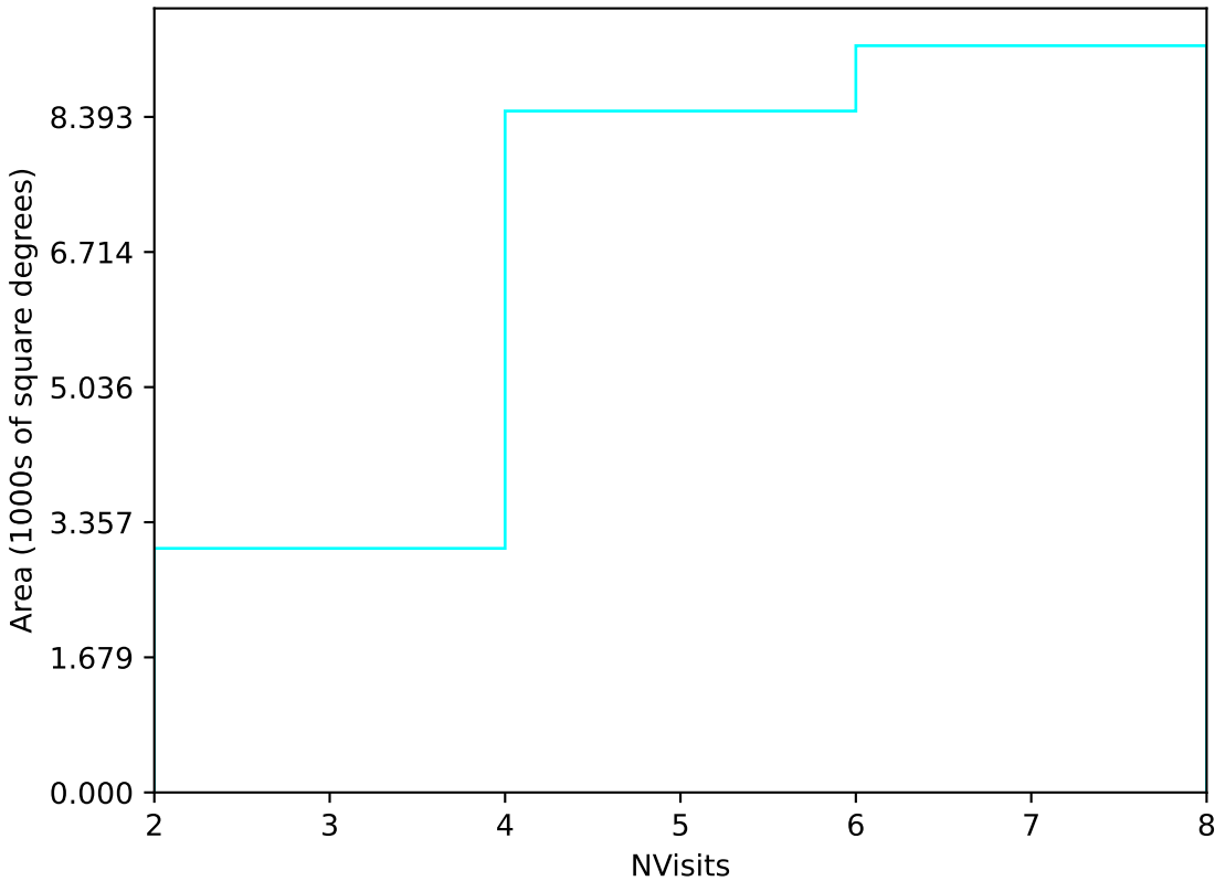
roll_uniform_early_half_mjdp0_v3.4_10yrs Yr 1 u band: NVisits
