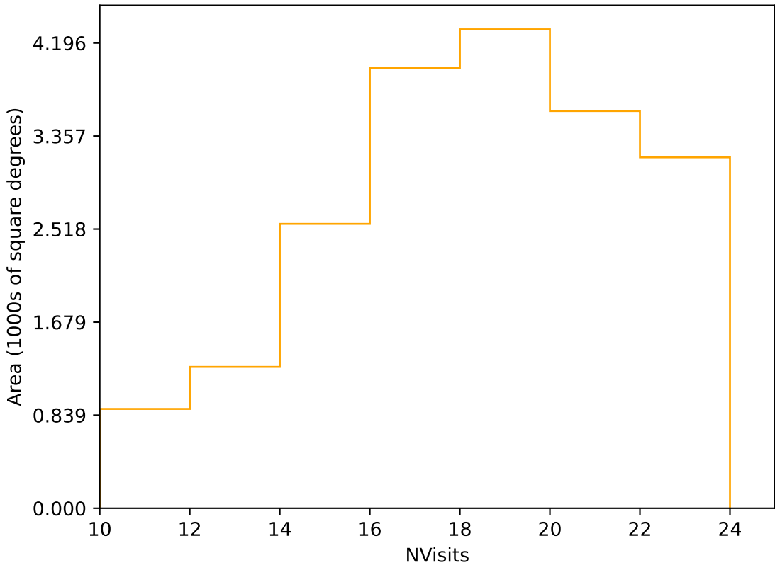
roll_uniform_early_half_mjdp0_v3.4_10yrs Yr 1 r band: NVisits
