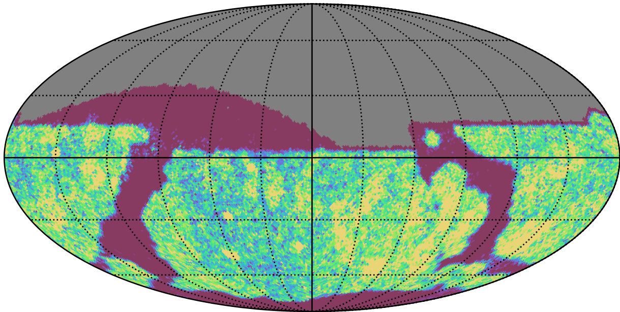
roll_uniform_early_half_mjdp0_v3.4_10yrs Yr 1 i band: NVisits
