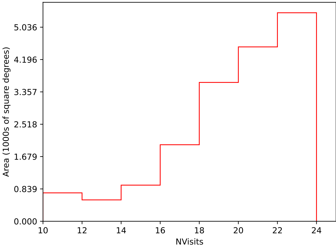
roll_uniform_early_half_mjdp0_v3.4_10yrs Yr 1 i band: NVisits
