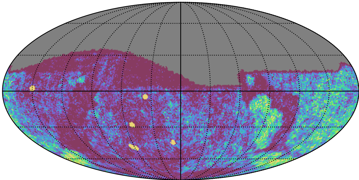
roll_uniform_early_half_mjdp0_v3.4_10yrs Yr 1 g band: NVisits
