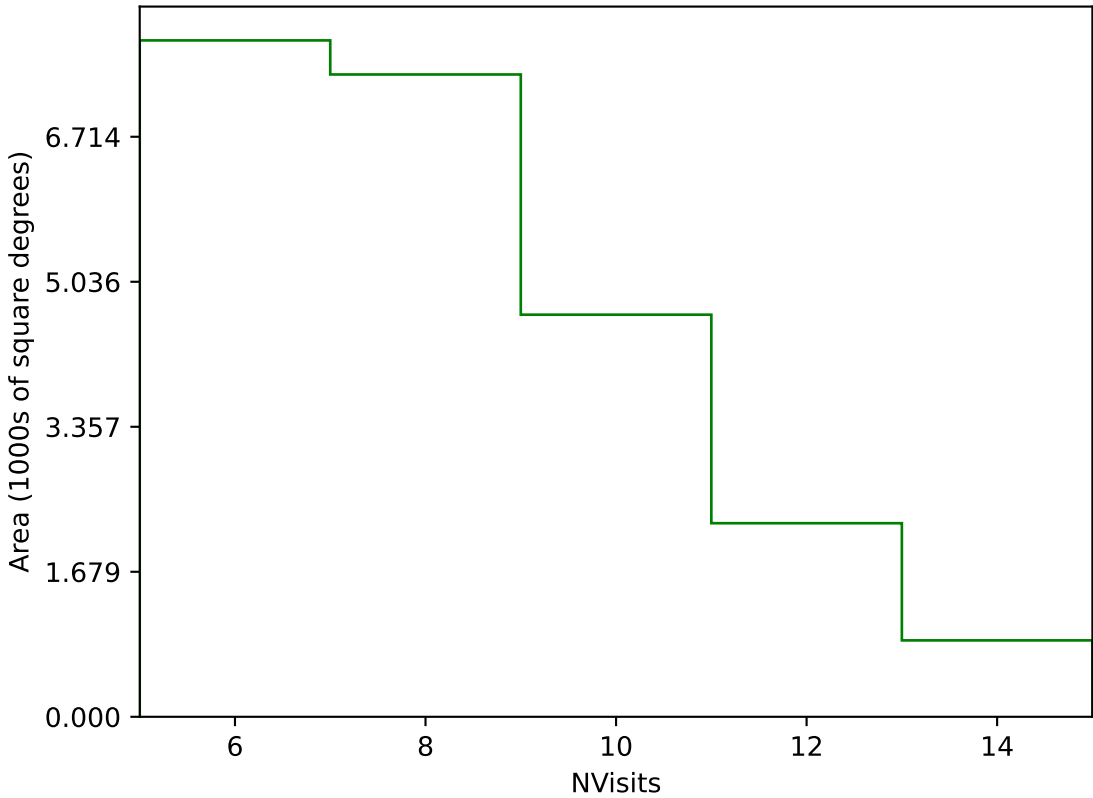
roll_uniform_early_half_mjdp0_v3.4_10yrs Yr 1 g band: NVisits
