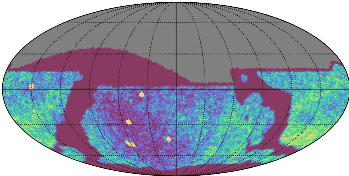
roll_uniform_early_half_mjdp0_v3.4_10yrs Yr 1 all bands: NVisits
