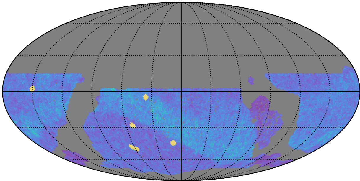
roll_uniform_early_half_mjdp0_v3.4_10yrs WFD z band: NVisits
