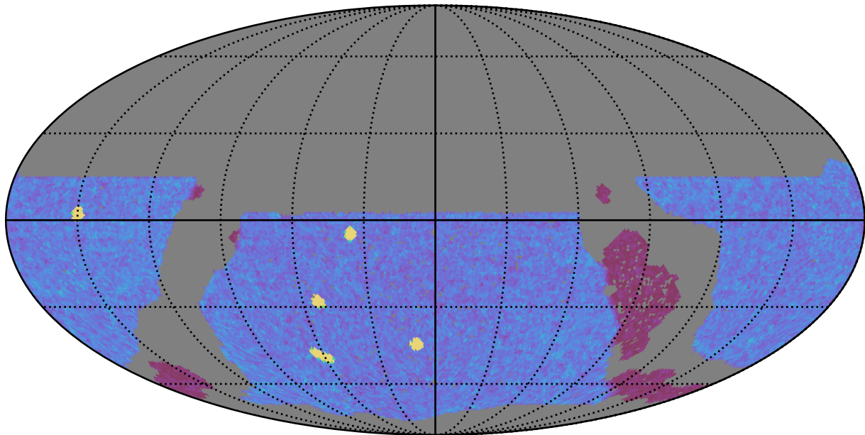
roll_uniform_early_half_mjdp0_v3.4_10yrs WFD y band: NVisits
