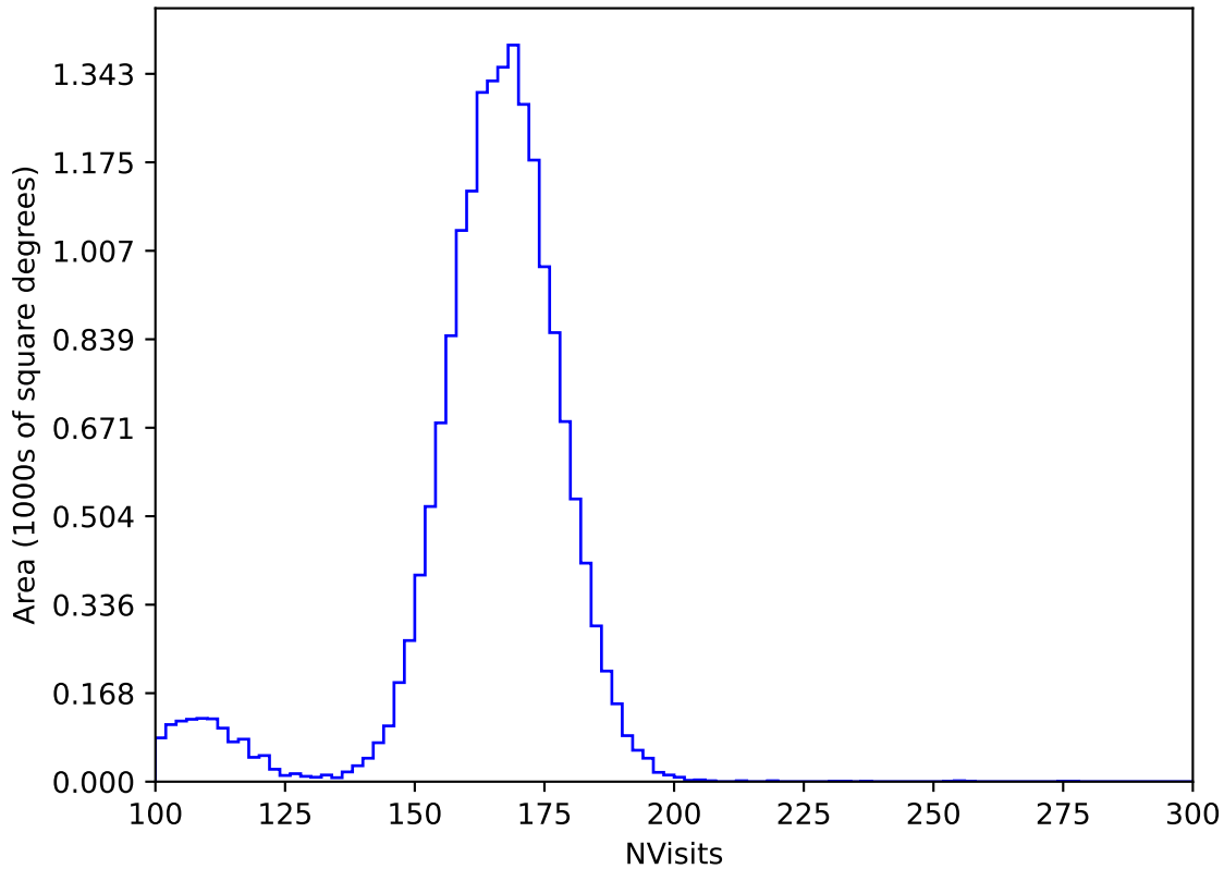
roll_uniform_early_half_mjdp0_v3.4_10yrs WFD y band: NVisits
