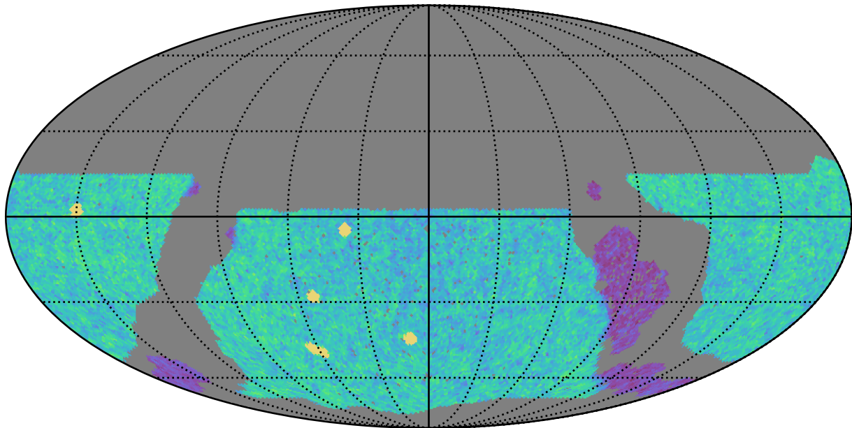
roll_uniform_early_half_mjdp0_v3.4_10yrs WFD u band: NVisits
