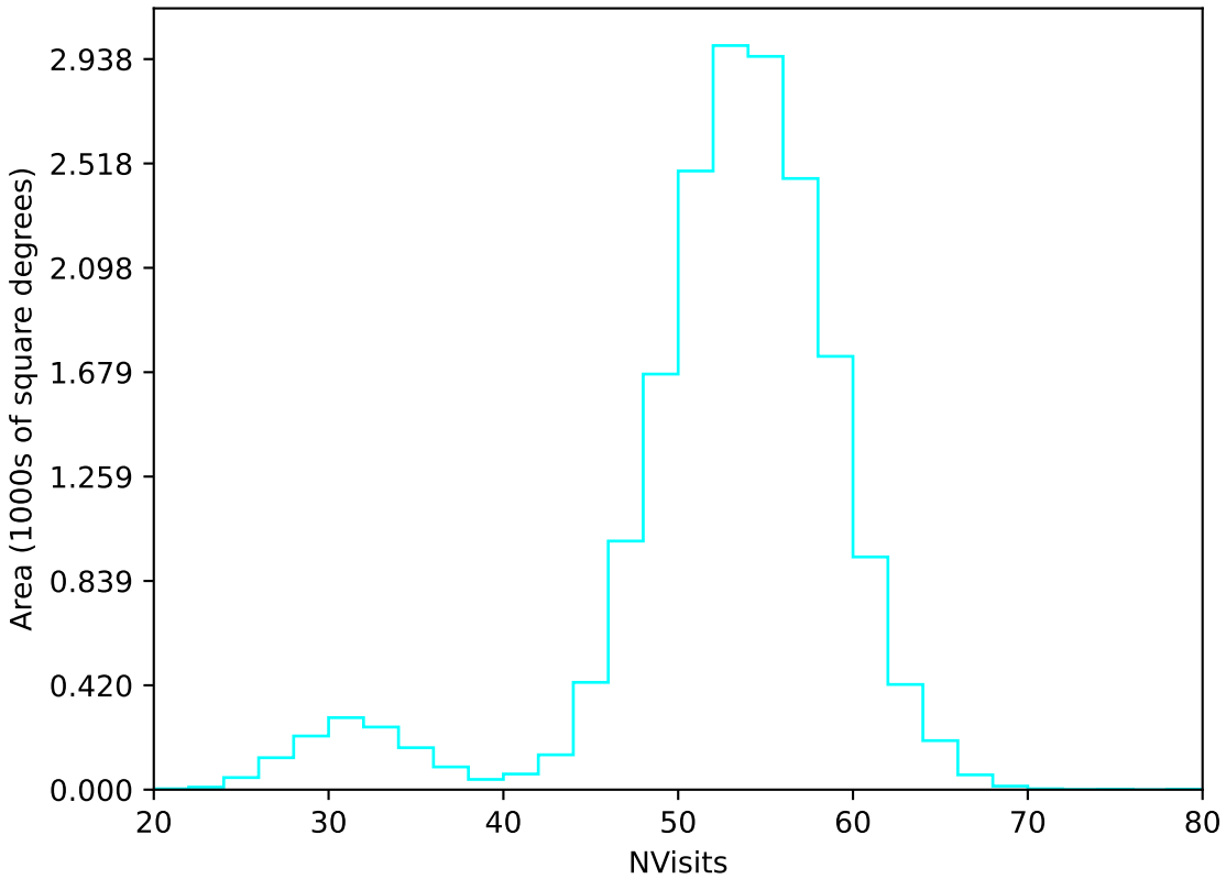
roll_uniform_early_half_mjdp0_v3.4_10yrs WFD u band: NVisits
