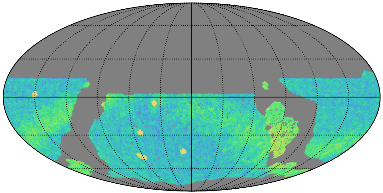
roll_uniform_early_half_mjdp0_v3.4_10yrs WFD r band: NVisits
