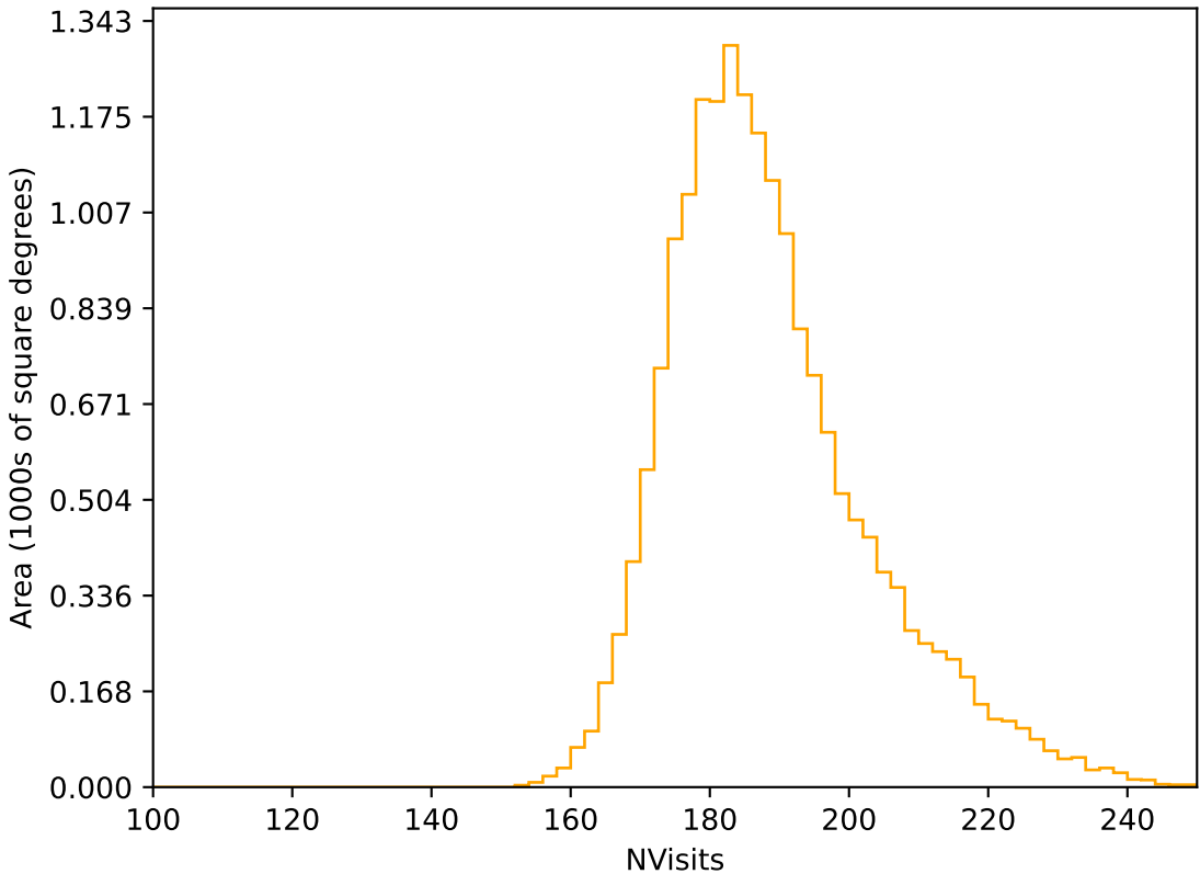
roll_uniform_early_half_mjdp0_v3.4_10yrs WFD r band: NVisits
