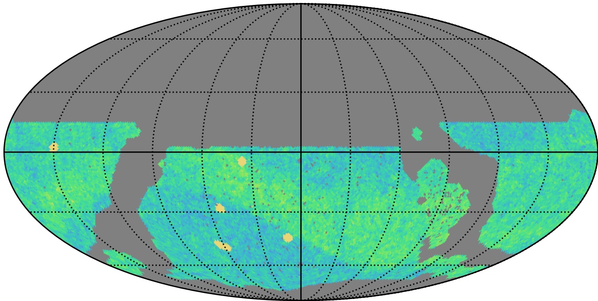
roll_uniform_early_half_mjdp0_v3.4_10yrs WFD i band: NVisits
