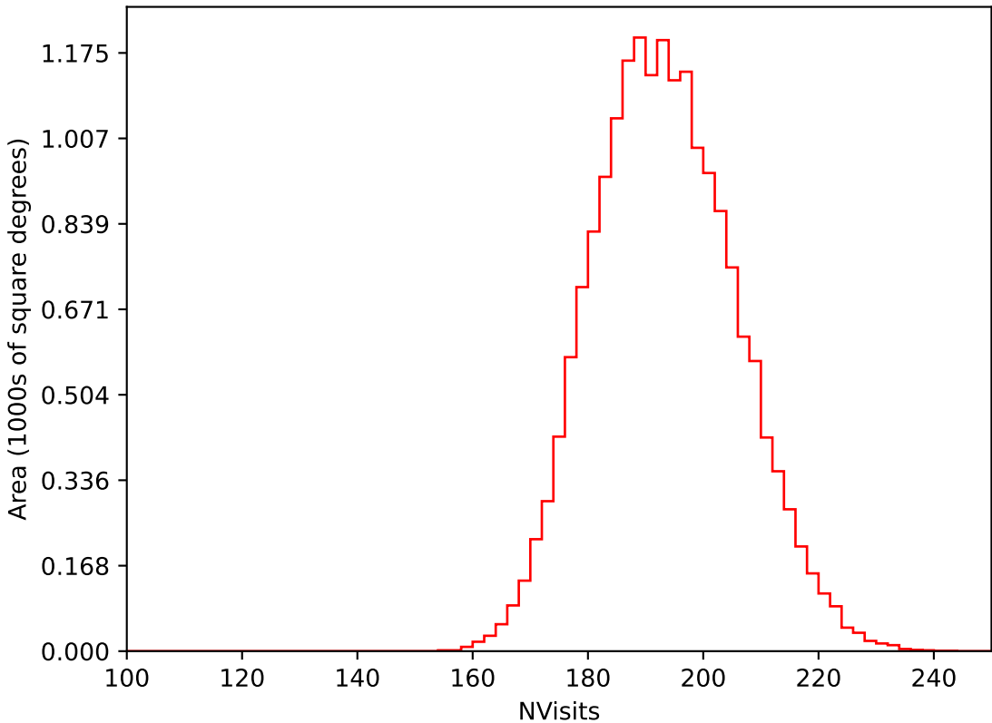
roll_uniform_early_half_mjdp0_v3.4_10yrs WFD i band: NVisits
