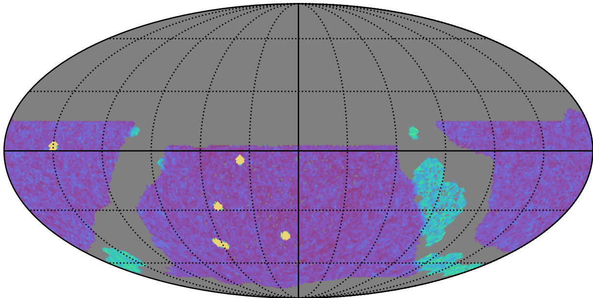
roll_uniform_early_half_mjdp0_v3.4_10yrs WFD g band: NVisits
