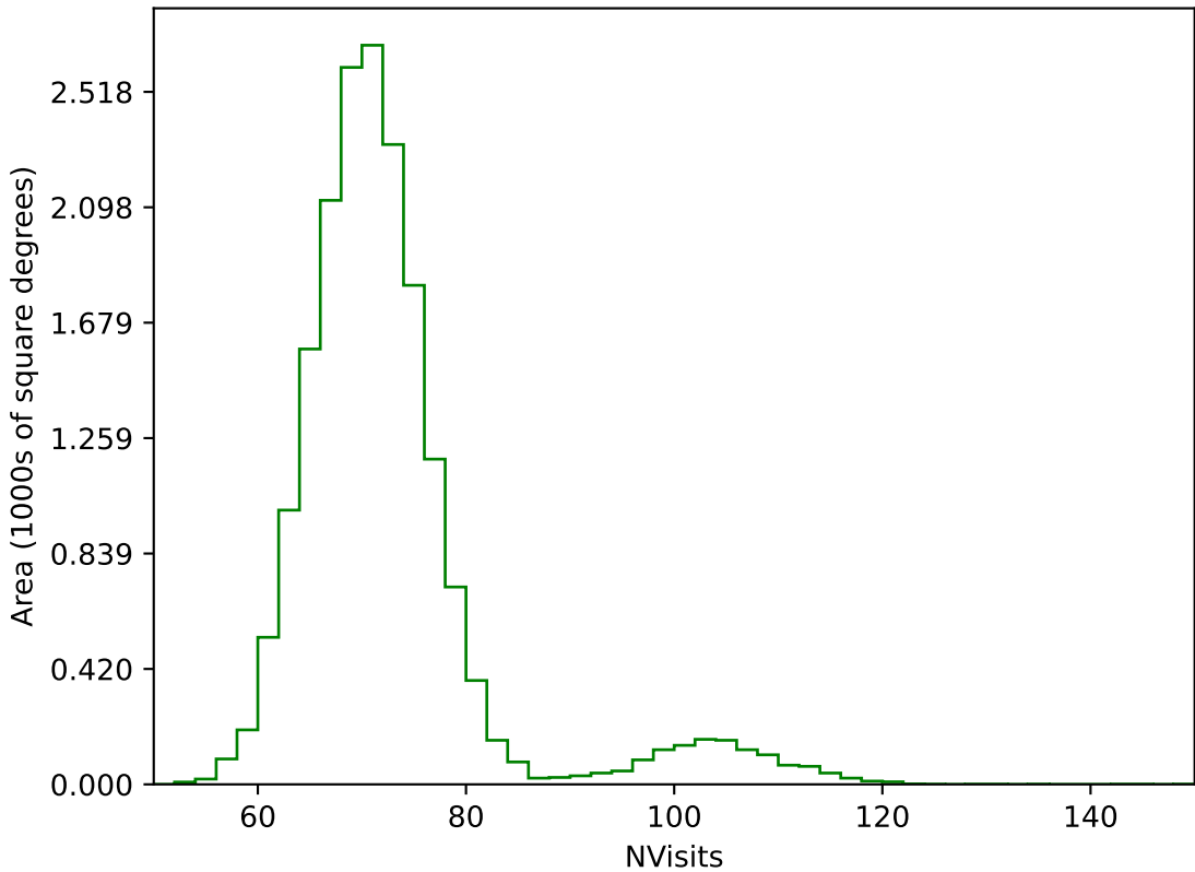
roll_uniform_early_half_mjdp0_v3.4_10yrs WFD g band: NVisits
