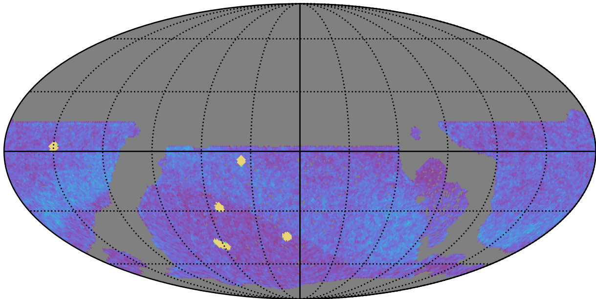
roll_uniform_early_half_mjdp0_v3.4_10yrs WFD all bands: NVisits
