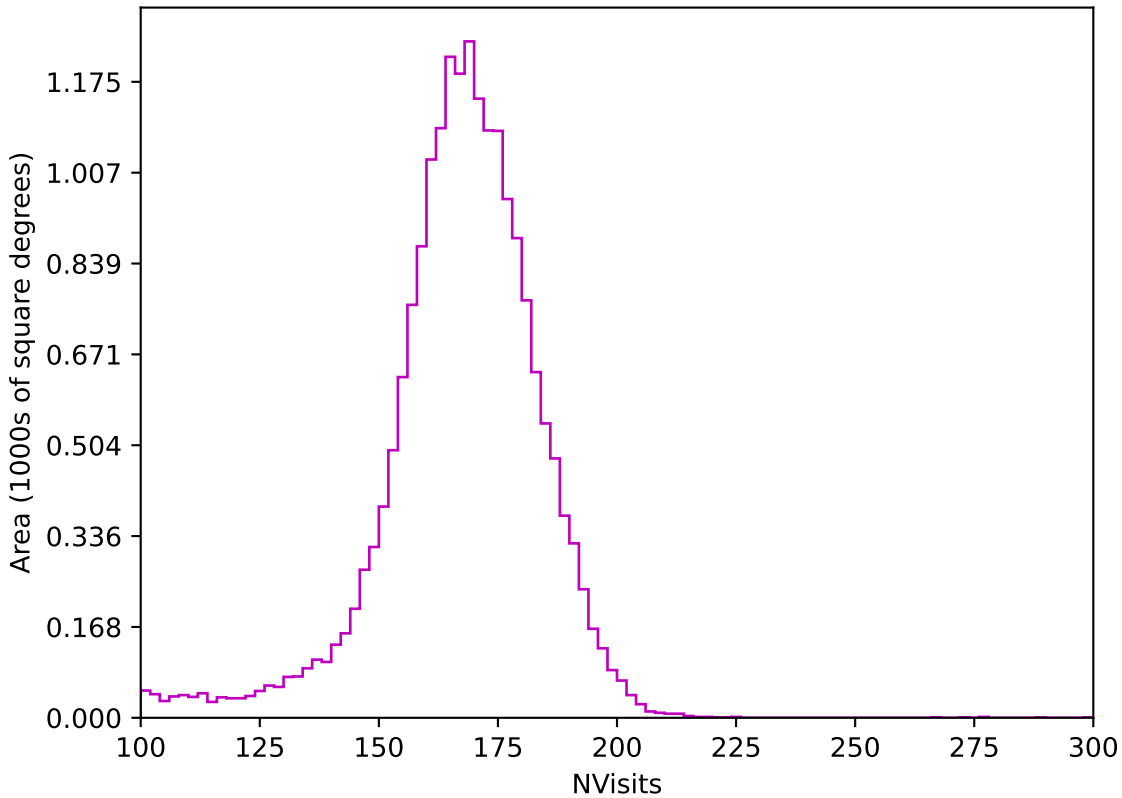
roll_uniform_early_half_mjdp0_v3.4_10yrs All sky z band: NVisits
