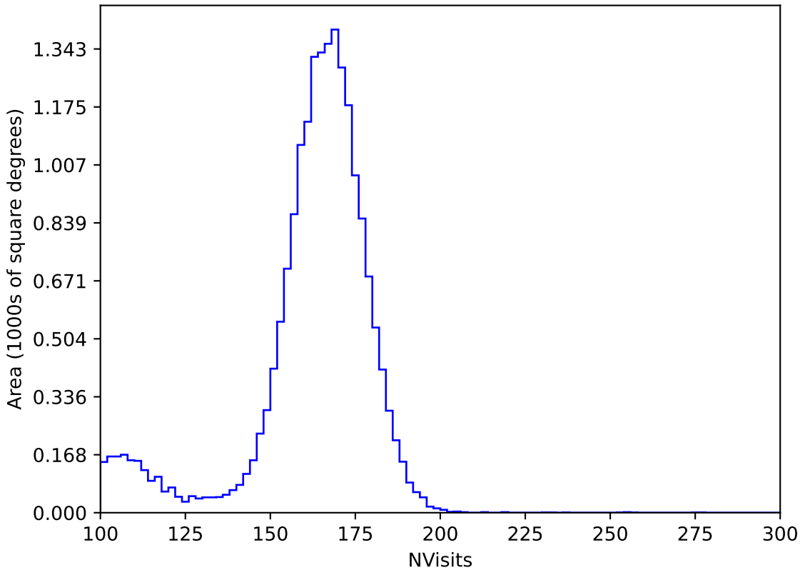
roll_uniform_early_half_mjdp0_v3.4_10yrs All sky y band: NVisits
