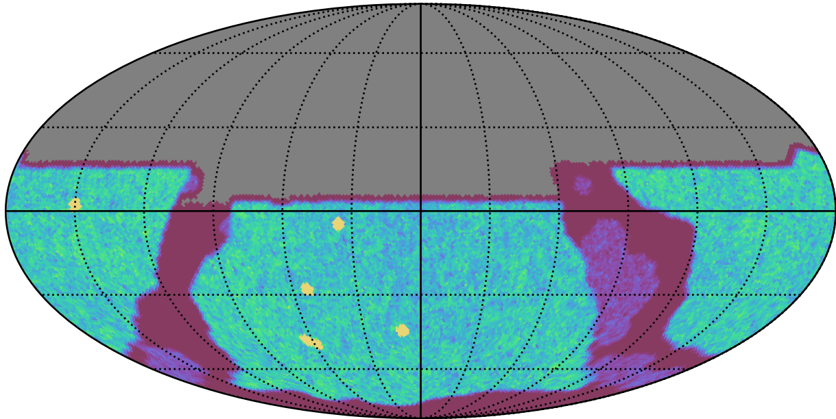
roll_uniform_early_half_mjdp0_v3.4_10yrs All sky u band: NVisits
