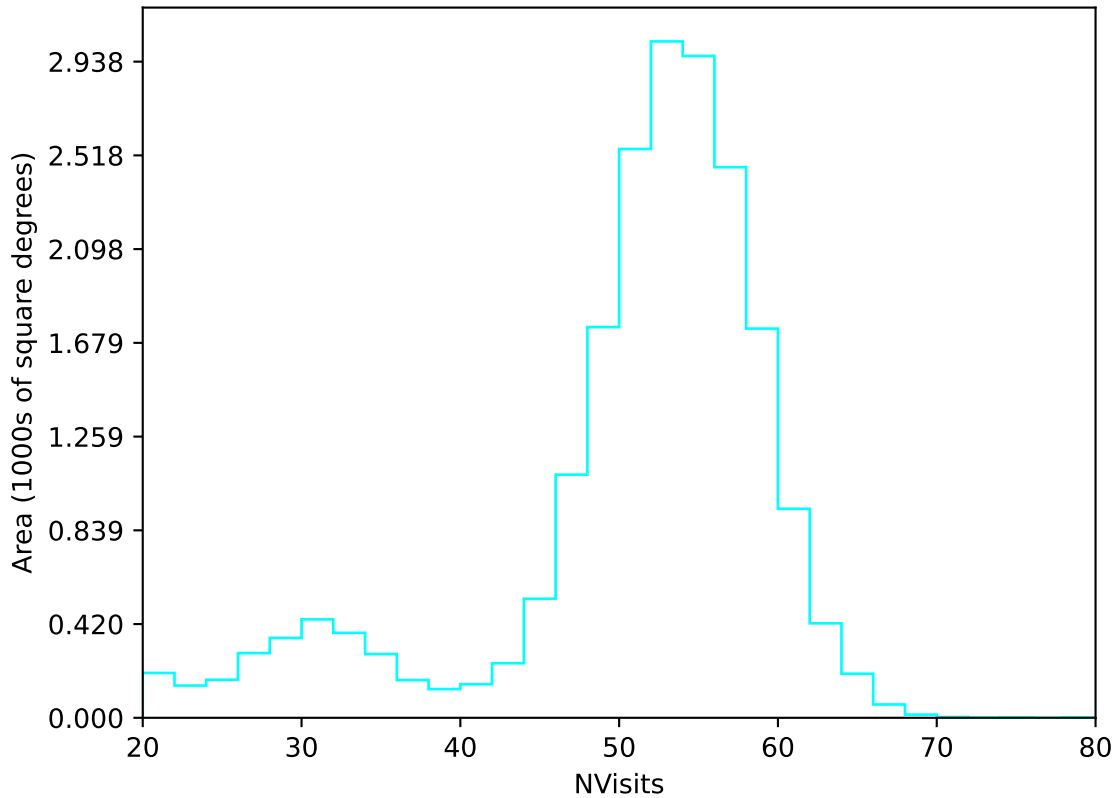
roll_uniform_early_half_mjdp0_v3.4_10yrs All sky u band: NVisits
