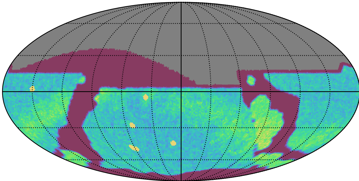
roll_uniform_early_half_mjdp0_v3.4_10yrs All sky r band: NVisits
