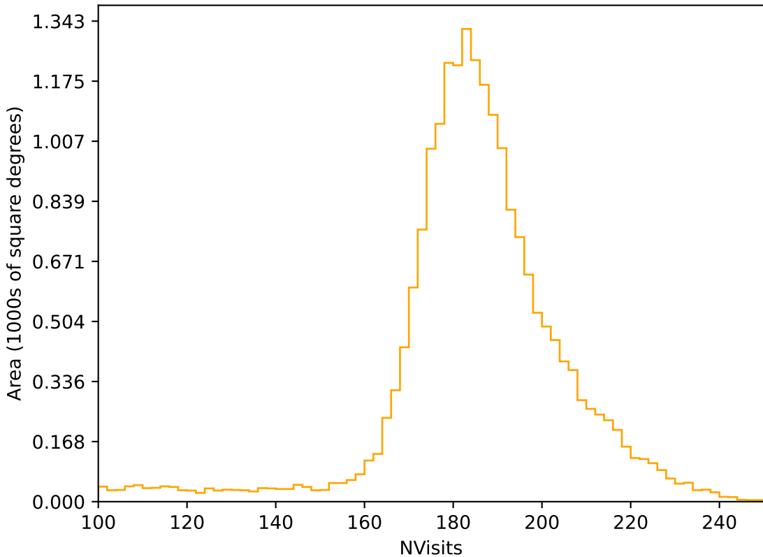
roll_uniform_early_half_mjdp0_v3.4_10yrs All sky r band: NVisits
