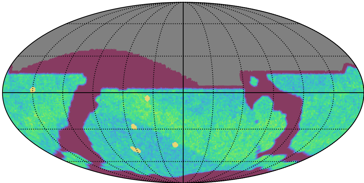
roll_uniform_early_half_mjdp0_v3.4_10yrs All sky i band: NVisits
