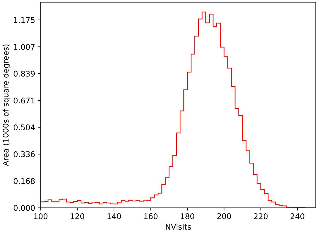
roll_uniform_early_half_mjdp0_v3.4_10yrs All sky i band: NVisits
