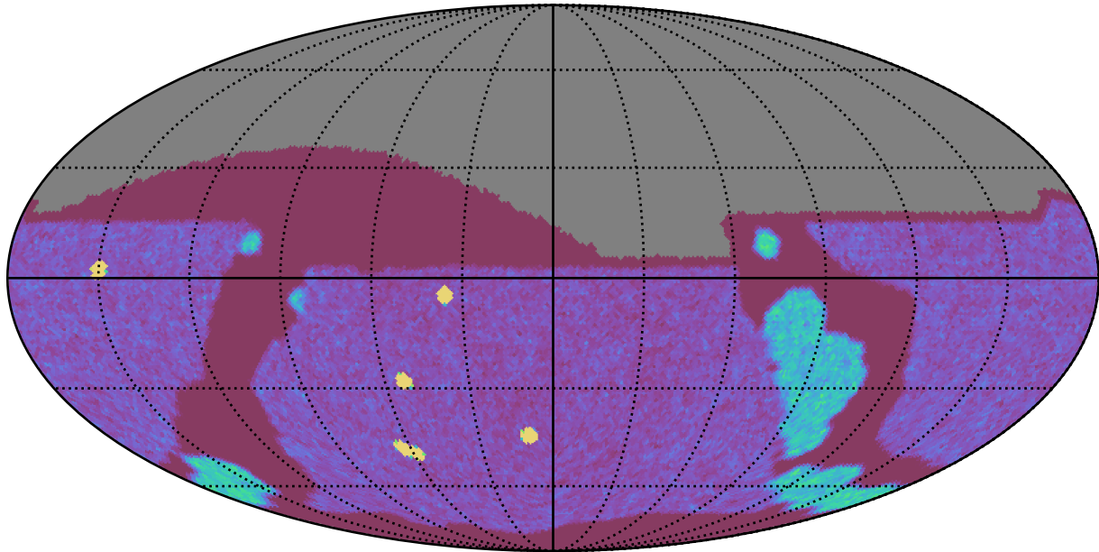
roll_uniform_early_half_mjdp0_v3.4_10yrs All sky g band: NVisits
