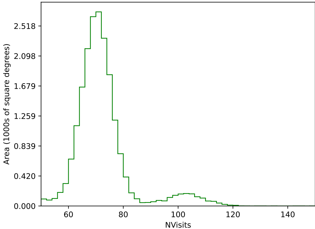
roll_uniform_early_half_mjdp0_v3.4_10yrs All sky g band: NVisits
