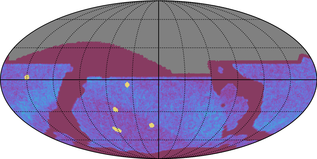
roll_uniform_early_half_mjdp0_v3.4_10yrs All sky all bands: NVisits
