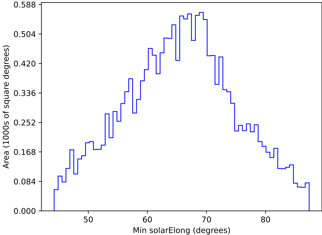
roll_uniform_early_half_mjdp0_v3.4_10yrs WFD y band: Min solarElong
