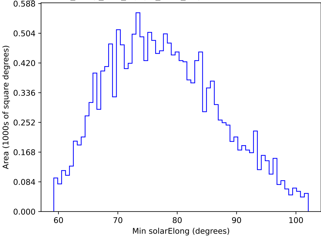
roll_uniform_early_half_mjdp0_v3.4_10yrs WFD u band: Min solarElong
