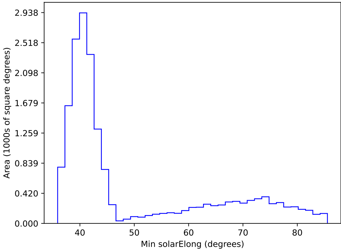
roll_uniform_early_half_mjdp0_v3.4_10yrs WFD i band: Min solarElong
