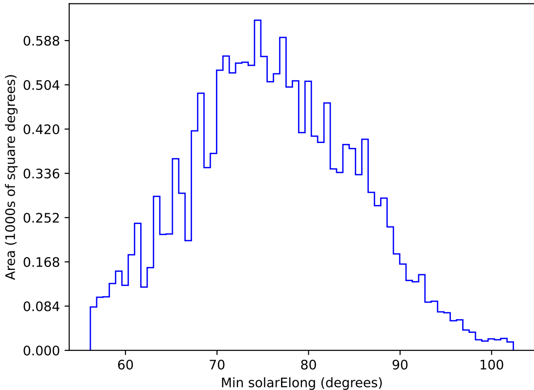
roll_uniform_early_half_mjdp0_v3.4_10yrs WFD g band: Min solarElong
