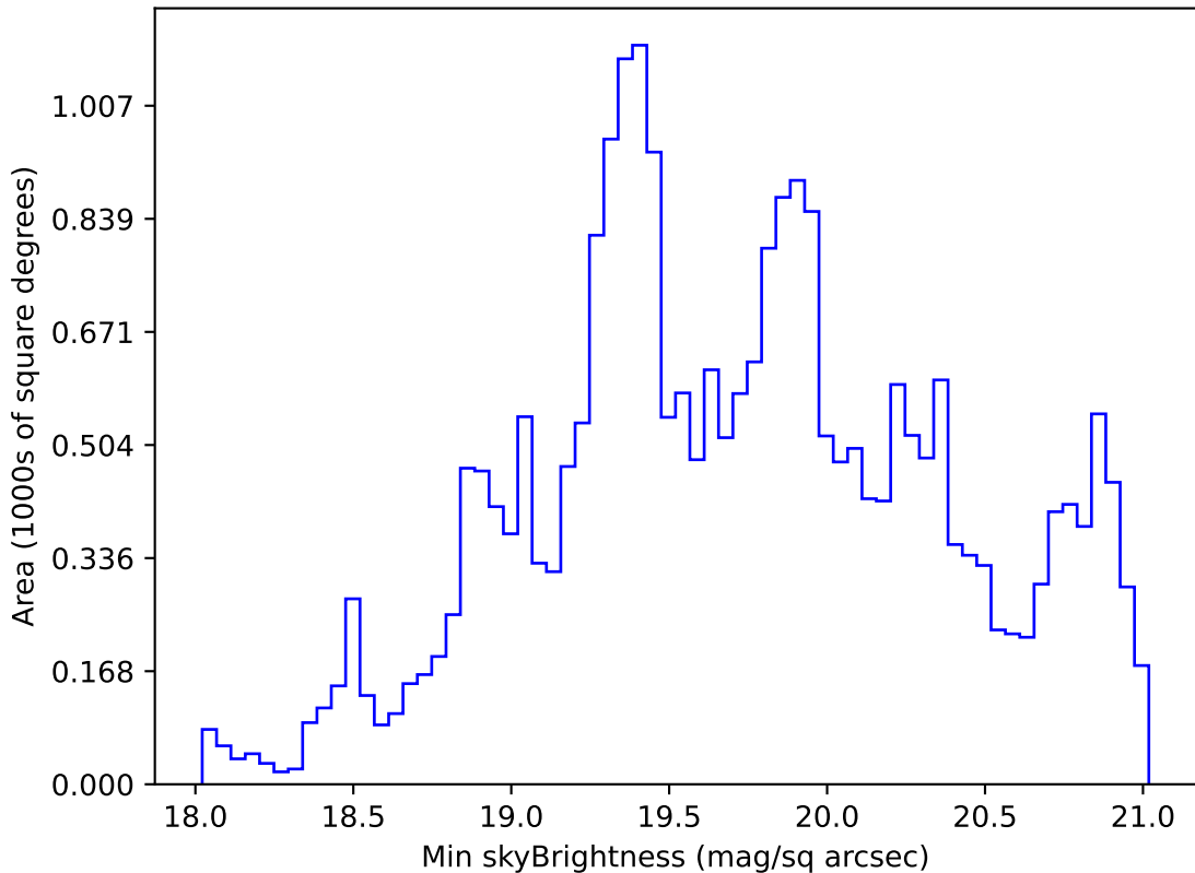
roll_uniform_early_half_mjdp0_v3.4_10yrs Yr 1 r band: Min skyBrightness
