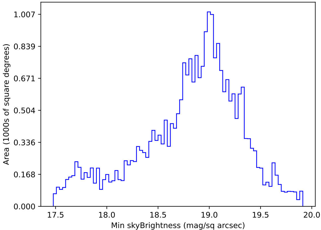
roll_uniform_early_half_mjdp0_v3.4_10yrs Yr 1 i band: Min skyBrightness
