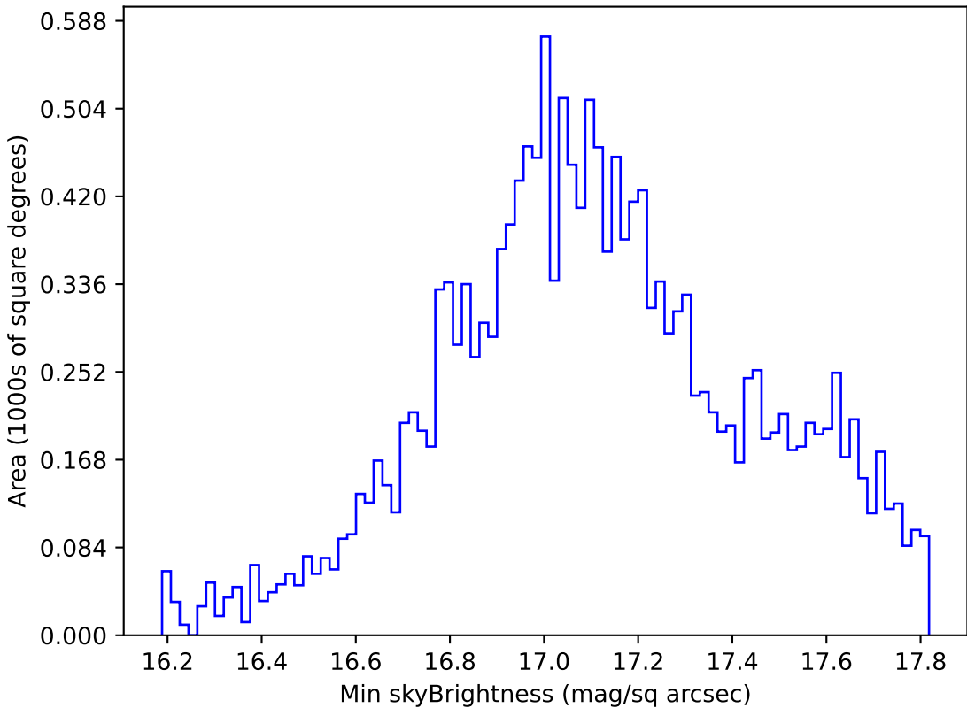
roll_uniform_early_half_mjdp0_v3.4_10yrs WFD y band: Min skyBrightness
