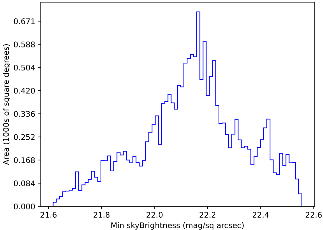
roll_uniform_early_half_mjdp0_v3.4_10yrs WFD u band: Min skyBrightness
