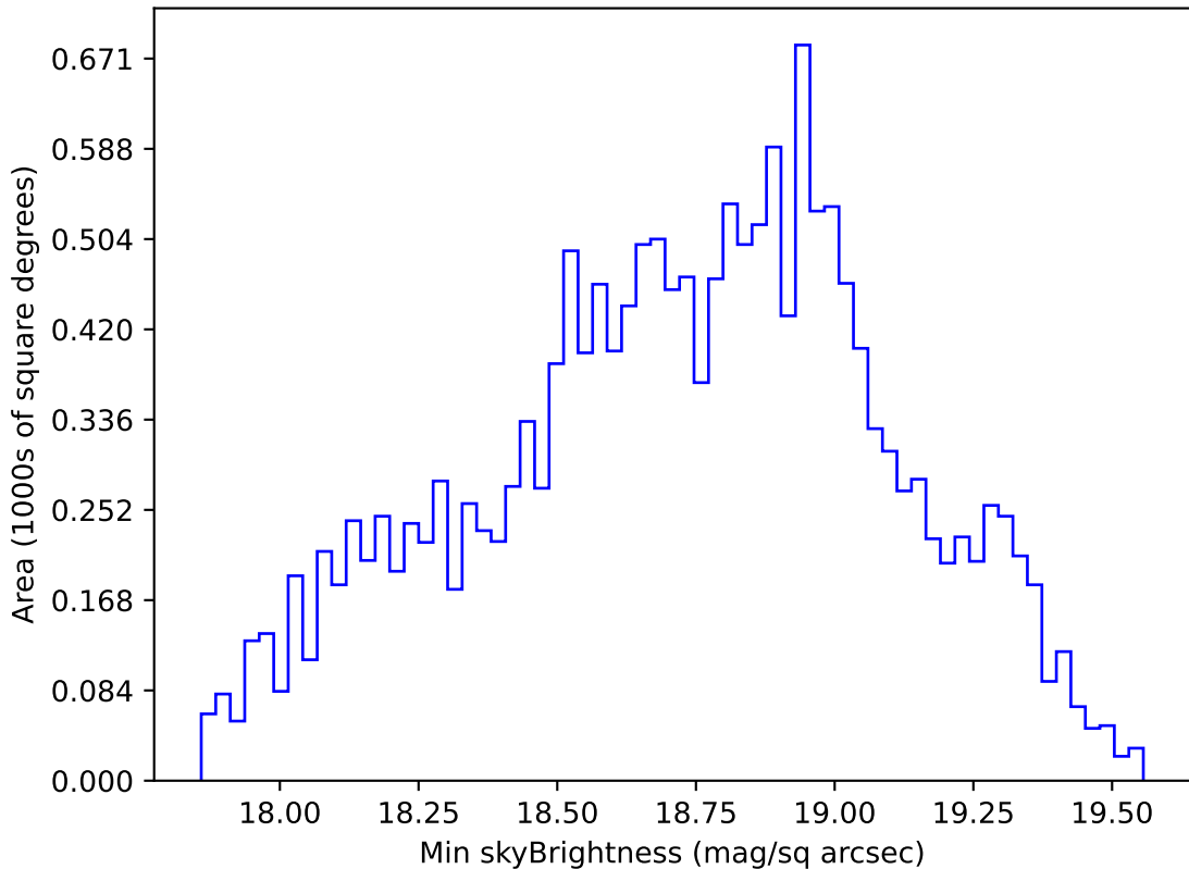
roll_uniform_early_half_mjdp0_v3.4_10yrs WFD r band: Min skyBrightness
