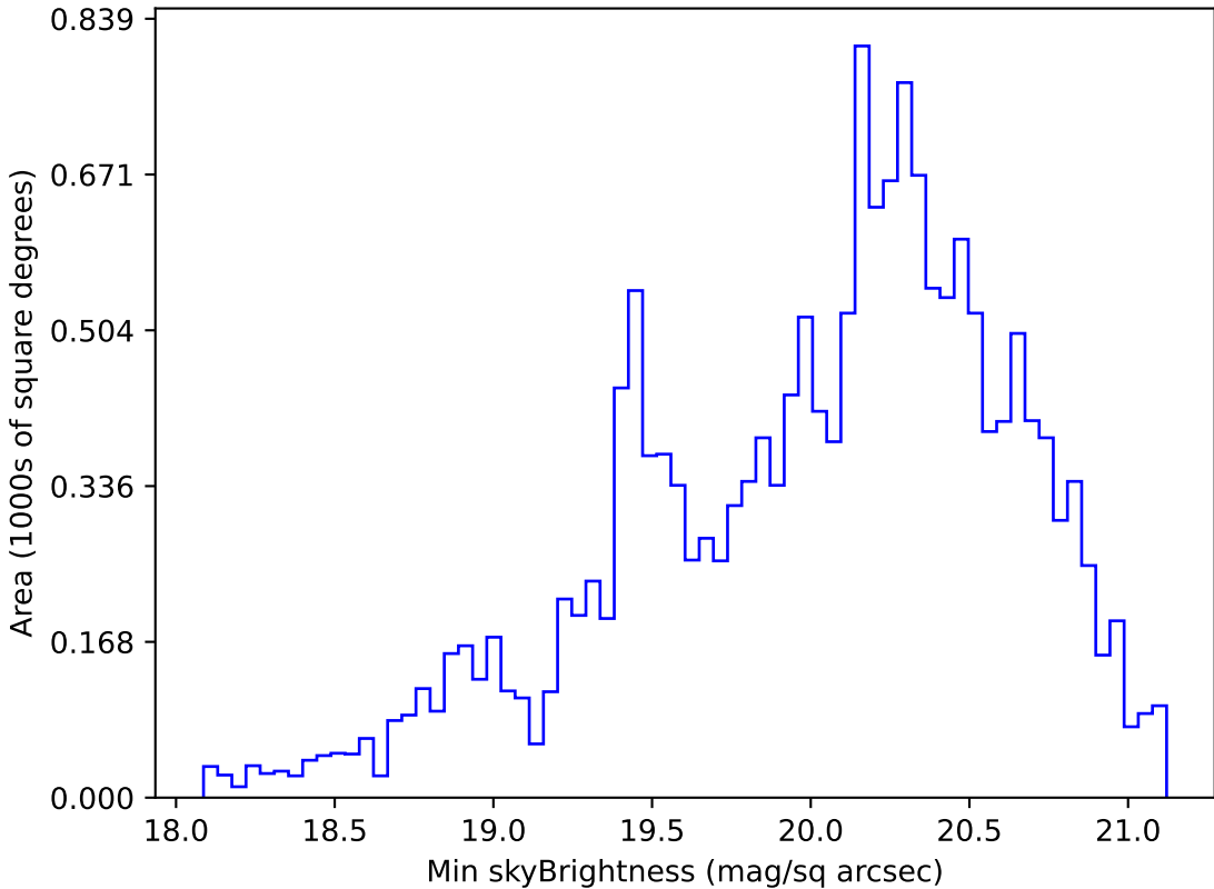
roll_uniform_early_half_mjdp0_v3.4_10yrs WFD g band: Min skyBrightness
