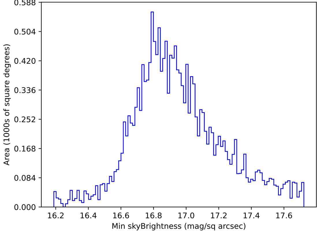
roll_uniform_early_half_mjdp0_v3.4_10yrs WFD all bands: Min skyBrightness
