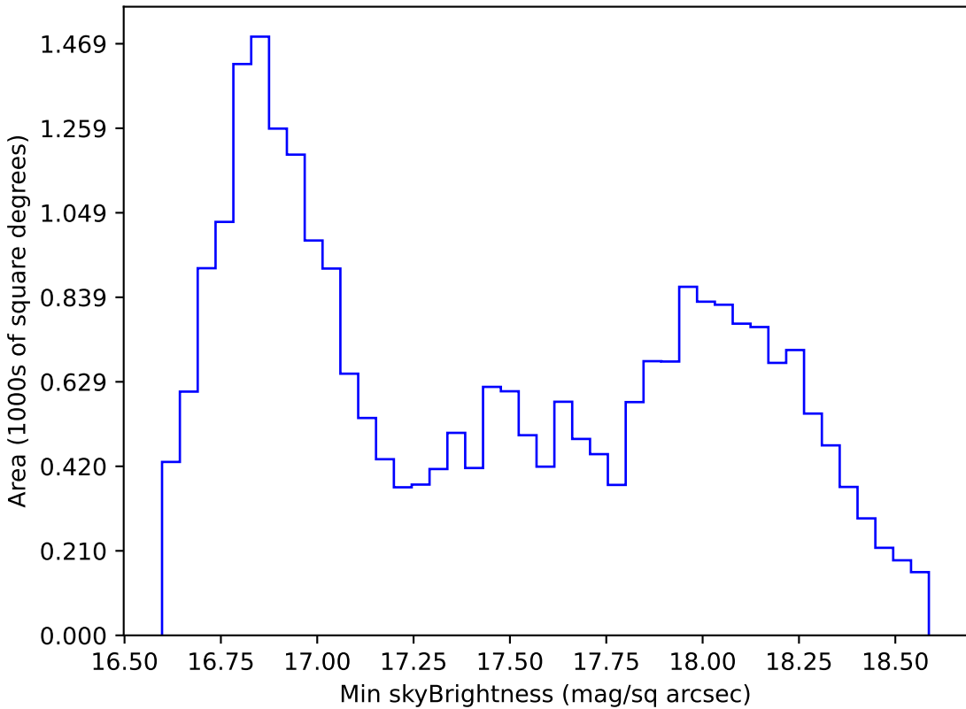
roll_uniform_early_half_mjdp0_v3.4_10yrs All sky z band: Min skyBrightness
