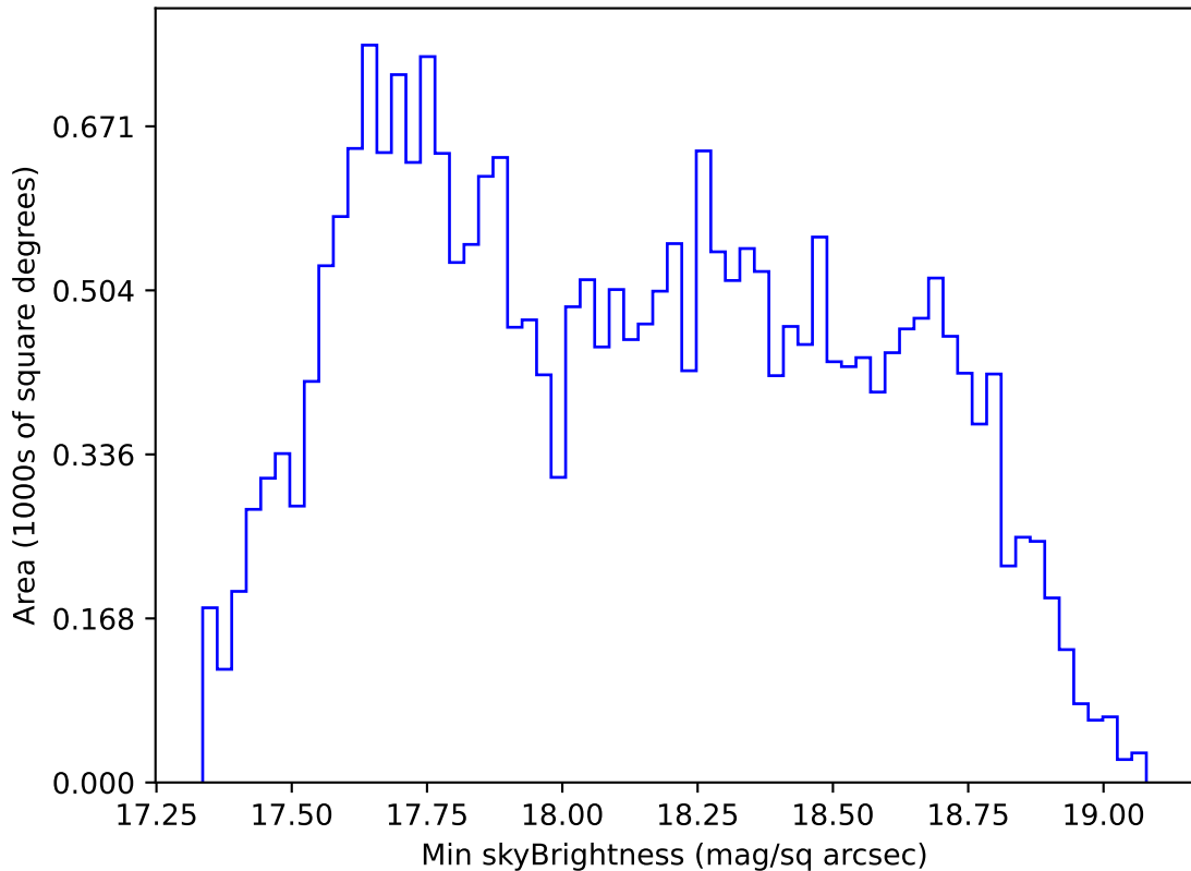
roll_uniform_early_half_mjdp0_v3.4_10yrs All sky i band: Min skyBrightness
