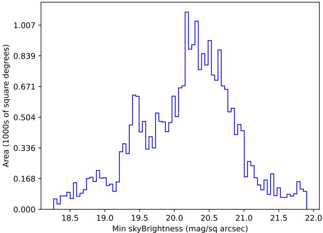
roll_uniform_early_half_mjdp0_v3.4_10yrs All sky g band: Min skyBrightness
