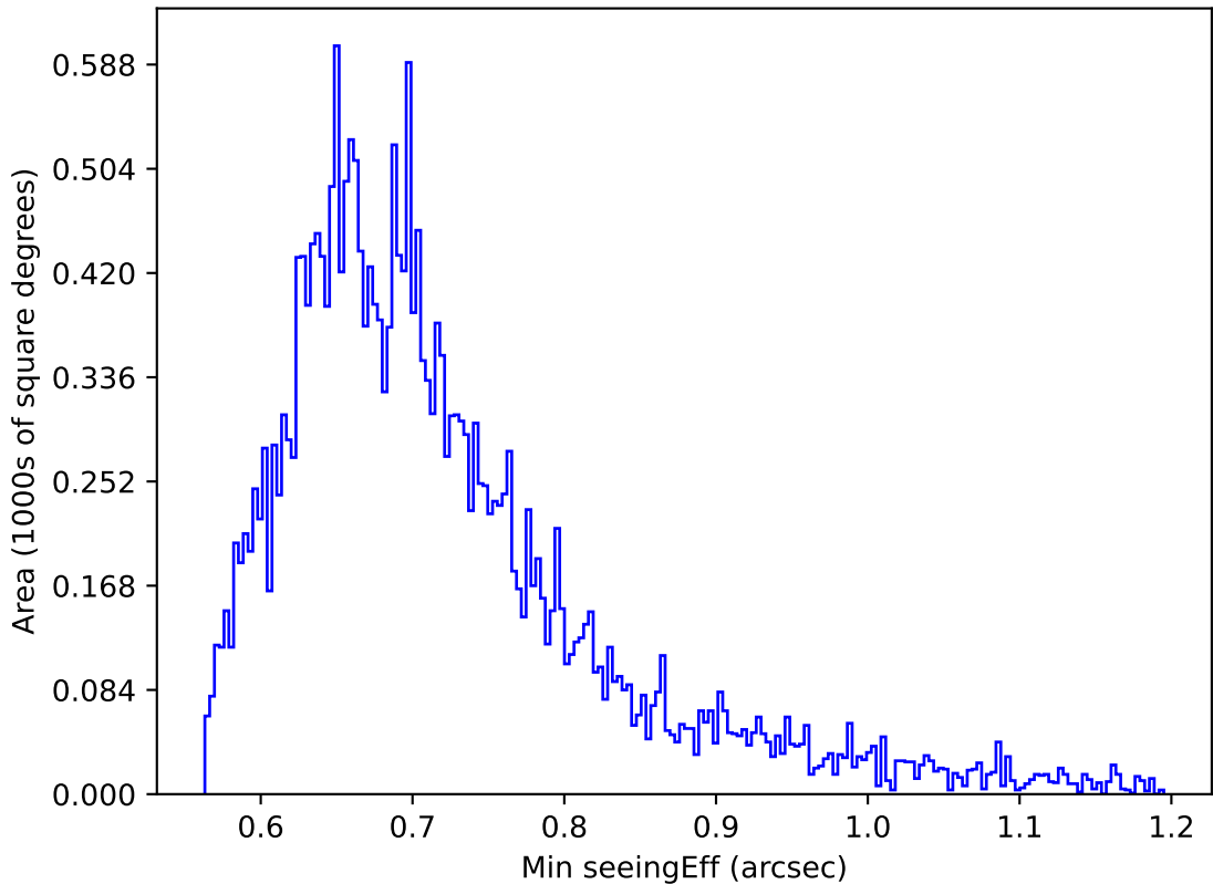
roll_uniform_early_half_mjdp0_v3.4_10yrs Yr 1 z band: Min seeingEff
